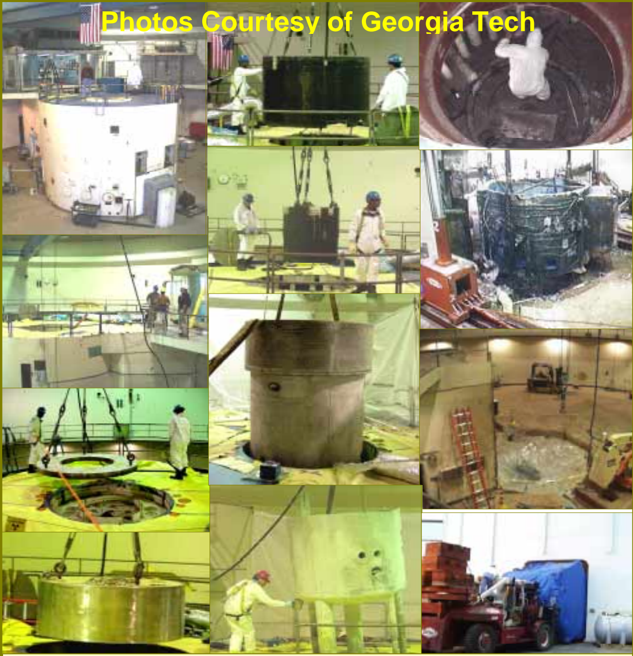
Disassembly and Decommissioning of the Georgia Tech Research Reactor 2000-2001
